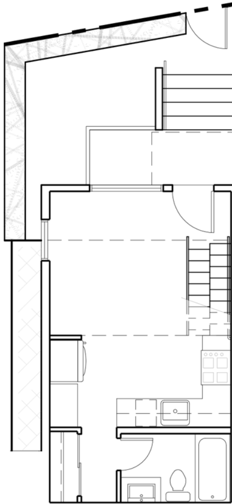
1st Floor
